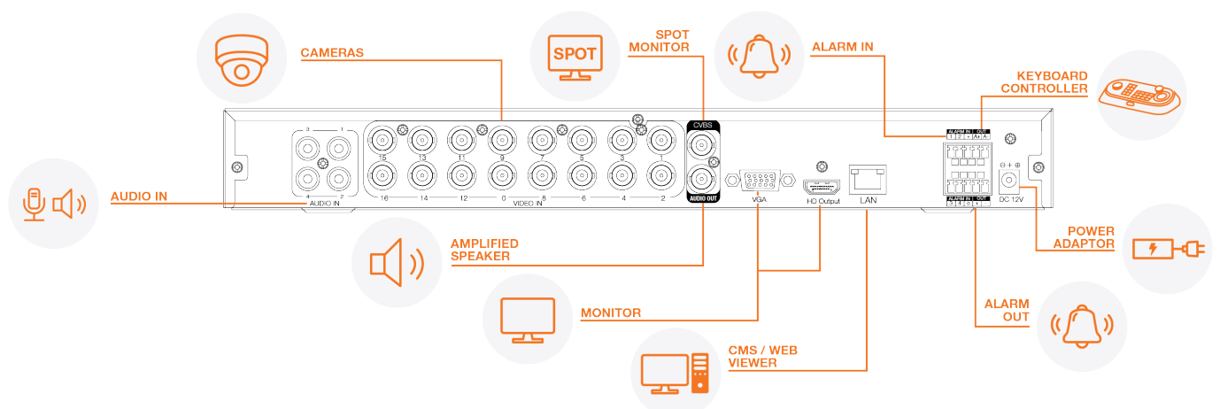
Figure 1-2 Name and Connection of each rear section
