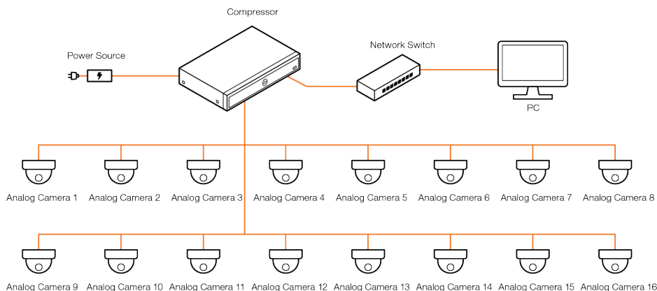
Figure 2-1 Connection map
